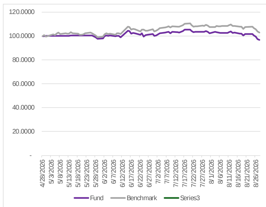
Cumulative Return
